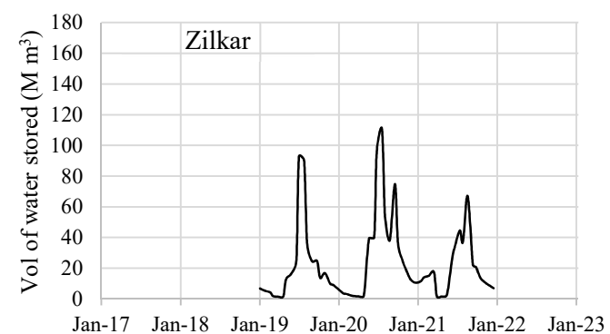
Figure S1: Time series of water volume stored in different haors.
