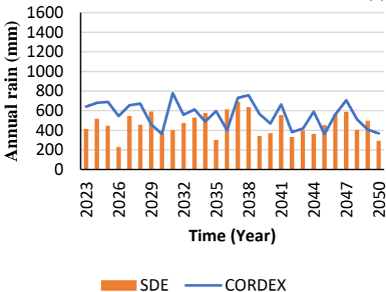
CNRM-CM5_rcp8.5
