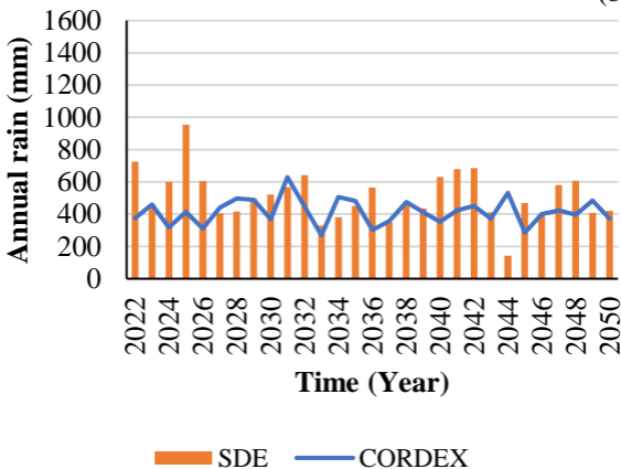
IPSL-CM5A-LR_rcp8.5
