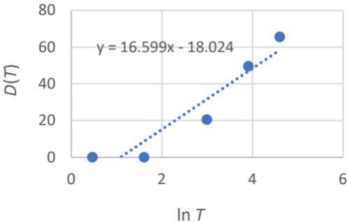
Damage cost as function of return period (log-linear graph)
