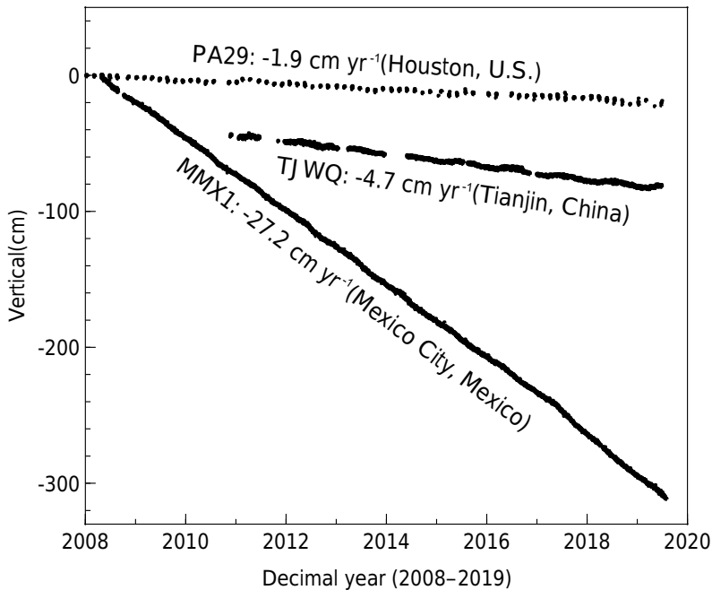
The most rapid subsidence in Tianjin, Houston, and Mexico City
