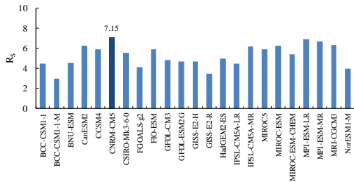
(a) Precipitation
