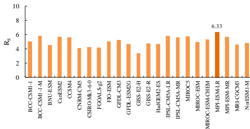
(c) Maximum air temperature
