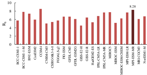
(b) Mean air temperature
