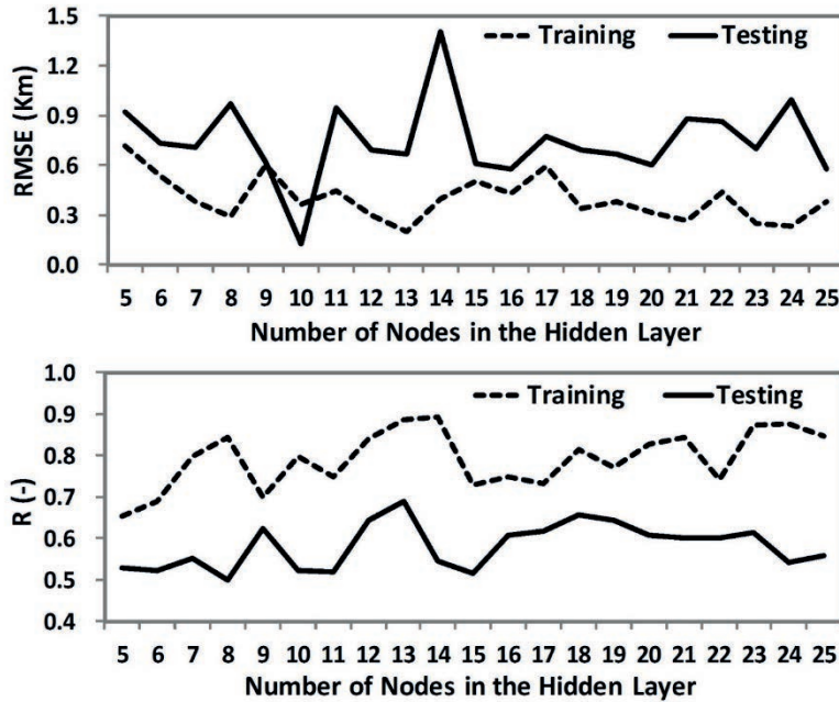
Fig. 1 The RMSE and correlation coefficient (R) of atmospheric visibility estimates for different numbers of nodes in the hidden layer.
